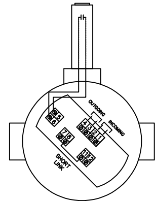
WIRING WITHOUT RESISTOR FIG. 7
