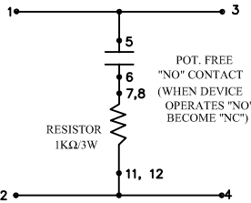
EQUIVALENT CIRCUIT FOR 2 WIRE CONVENTIONAL SYSTEM FIG. 2
