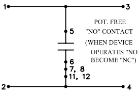
EQUIVALENT CIRCUIT FIG. 1
