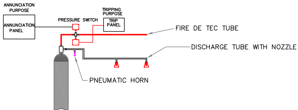
SCHEME EXPLAINING FIRE DETECTION AND EXTINGUISHING SYSTEM WITHOUT ANY EXTERNAL ELECTRICAL POWER
