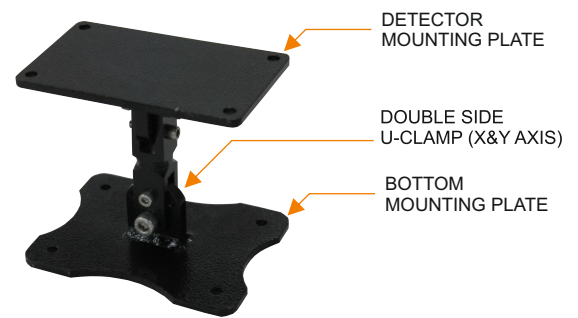
IHMB01-XY SWIVEL MOUNTING BASE
